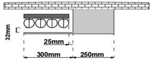
275 X 1800 ULA UNIVERSAL HANGER MODEL 3 R
