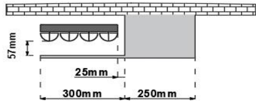
275 X 1800 BIRGI UNIVERSAL HANGER MODEL 3 R
