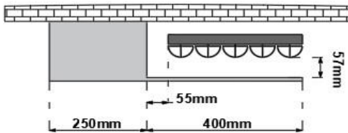
345 X 1800 BIRGI UNIVERSAL HANGER MODEL 2 L
