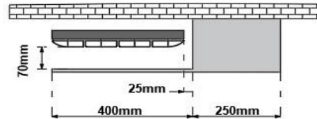
375 X 1800 SELANIK UNIVERSAL HANGER MODEL 2 R
