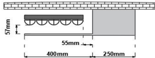
345 X 1800 BIRGI UNIVERSAL HANGER MODEL 2 R
