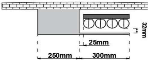
275 X 1800 ULA UNIVERSAL HANGER MODEL 3 L
