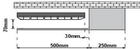
470 X 1800 SELANIK UNIVERSAL HANGER MODEL 1 R
