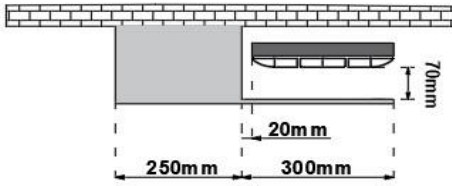
280 X 1800 SELANIK UNIVERSAL HANGER MODEL 3 L
