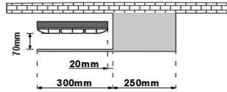
280 X 1800 SELANIK UNIVERSAL HANGER MODEL 3 R
