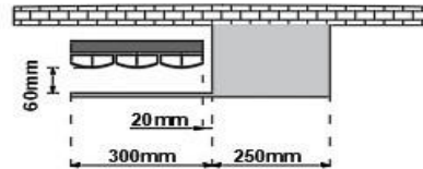
280 X 1800 KAVALA UNIVERSAL HANGER MODEL 3 R
