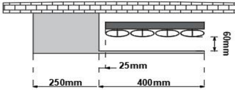
375 X 1800 SEREZ UNIVERSAL HANGER MODEL 2 L
