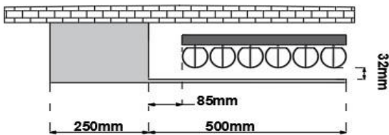
415 X 1800 ULA UNIVERSAL HANGER MODEL 1 L
