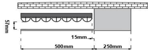
485 X 1800 BIRGI UNIVERSAL HANGER MODEL 1 R
