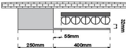
345 X 1800 ULA UNIVERSAL HANGER MODEL 2 L
