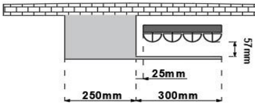
275 X 1800 BIRGI UNIVERSAL HANGER MODEL 3 L
