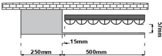
485 X 1800 BIRGI UNIVERSAL HANGER MODEL 1 L
