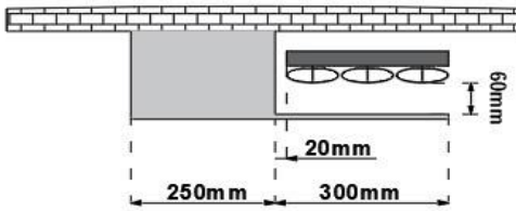
280 X 1800 SEREZ UNIVERSAL HANGER MODEL 3 L
