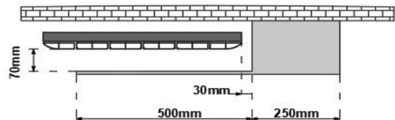
565 X 1800 SELANIK UNIVERSAL HANGER MODEL 1 R
