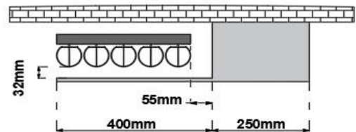
345 X 1800 ULA UNIVERSAL HANGER MODEL 2 R
