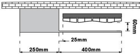
375 X 1800 CUNDA UNIVERSAL HANGER MODEL 2 L
