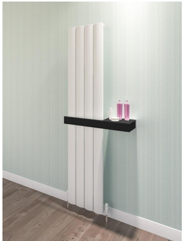
375 x 1800 Kavala Radiator with Universal Towel Hanger Model 2 Right
